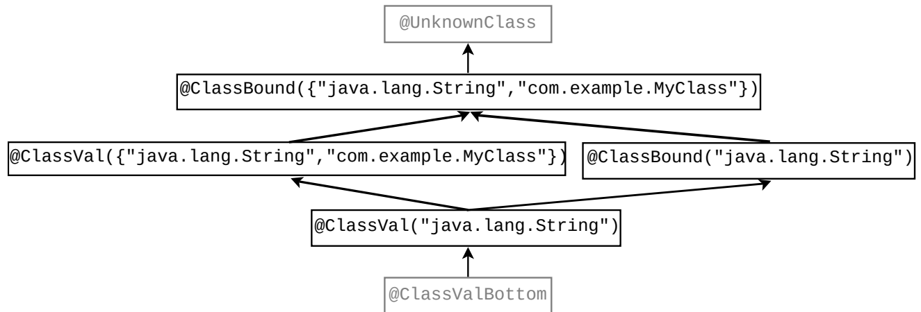
Figure 25.1: Partial type hierarchy for the ClassVal type system. The type qualifiers in gray ( @UnknownClass and @ClassValBottom ) should never be written in source code; they are used internally by the type system.
