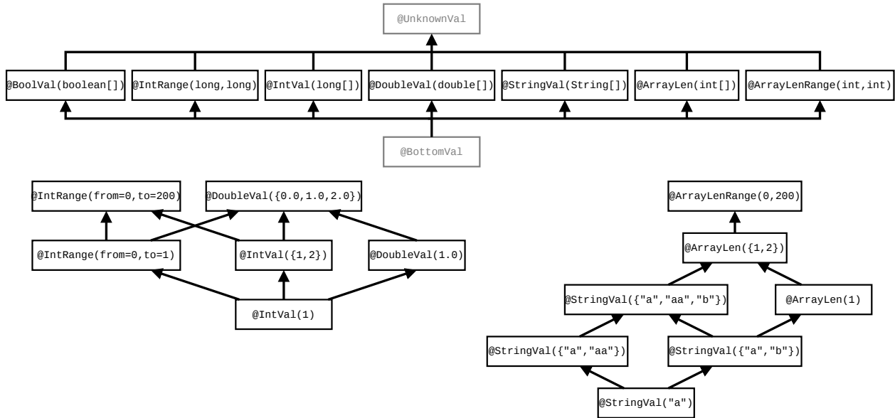
Figure 22.1: At the top, the type qualifier hierarchy of the Constant Value Checker annotations. The first four qualifiers are applicable to primitives and their wrappers; the next to Strings , and the final two to arrays. Qualifiers in gray are used internally by the type system but should never be written by a programmer. At the bottom are examples of additional subtyping relationships that depend on the annotations' arguments.
