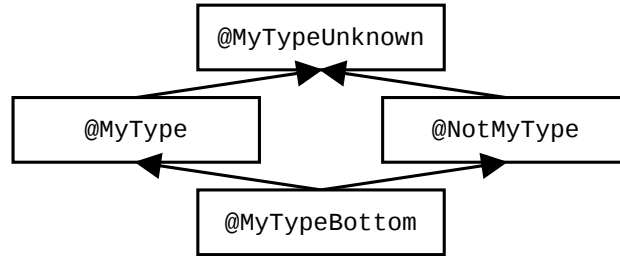
Figure 24.1: Type system for a type alias or typedef type system. The type system designer may choose to omit some of these types, but this is the general case. The type system designer’s choice of defaults affects the interpretation of unannotated code, which affects the guarantees given for unannotated code.
